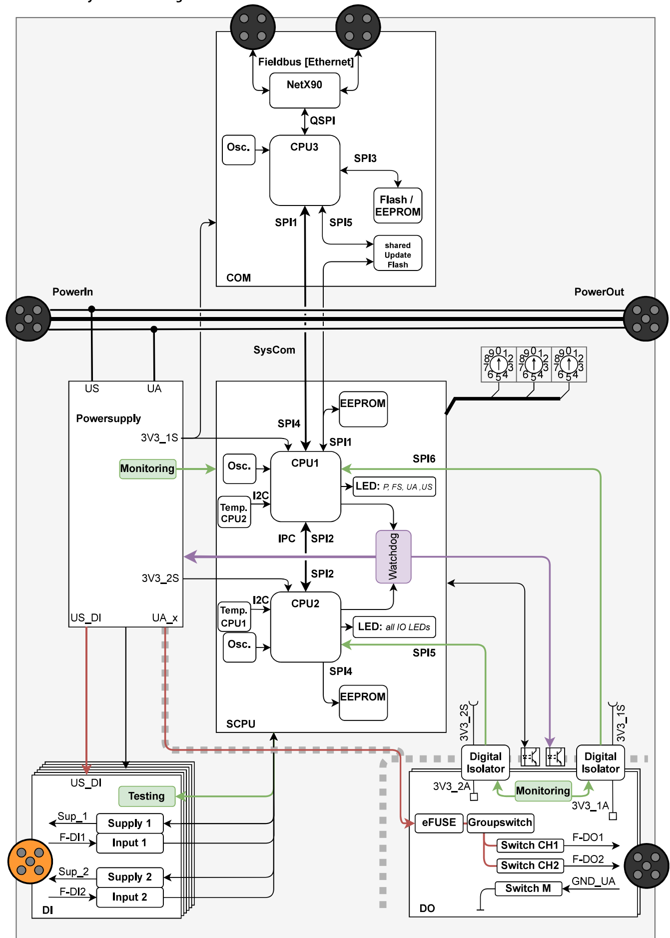
SRIO-10248 - System Block Diagramm
